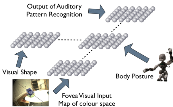
Figure 3: The label learning model architecture: self-organising maps are used to map the colour, shape, word and body spaces, with associative links formed (in a Hebbian-like manner) between peaks of activation in each map.
