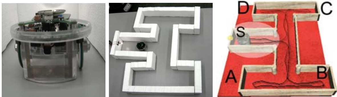
Figure 4. Left: The e-puck robot developed at EPFL, Switzerland ( http://www.e-puck.org/ ). Centre: The environment which have a size of 52cm by 60cm. The light produced by the light bulb located on the left side of the central corridor cannot be perceived from the other two corridors. Right: The motor trajectory produced by the robot during a complete lap of the environment.
