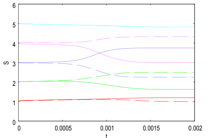
Fig. 2. Time evolution of the two components of the modeling fields in the case of N=5 objects. The weights a_i are chosen so as to mimic the co-occurrence frequency of objects and words in the cross situational learning scenario of Fig. 1. The second component, associated to the label of the word, is represented by a solid line and the first component, associated to the object, is represented by a dashed line. The M=5 different modeling fields are represented by different colors. The initial condition is a small perturbation of the correct object-word mapping.
