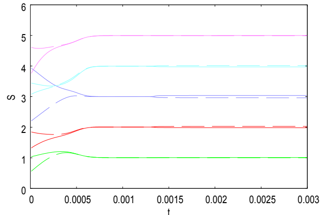
Fig. 3. Time evolution of the two components of the modeling fields in the case of N=5 objects. The weights a_i are chosen so as to model the learning with noise situation. We set a_i = 100 for the N examples of the form (n,n) and a_i = 1 for the other N(N-1) examples. The conventions for line color and style are the same as in Fig. 2. The initial condition for each component was chosen randomly in the range [0, N] .
