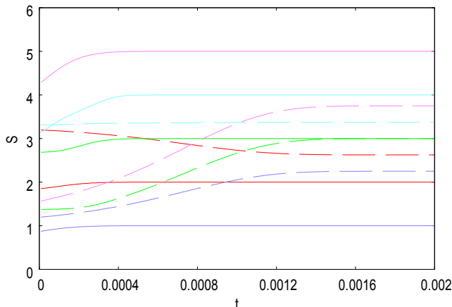
Fig. 4. Time evolution of the first (dashed line) and third (solid lines) entries of the modeling fields in the context-word input representation. The second entry (not shown in the figure) becomes identical to the first entry for t > 0.0012 . The initial condition for each component was chosen randomly in the range [0, N] .
