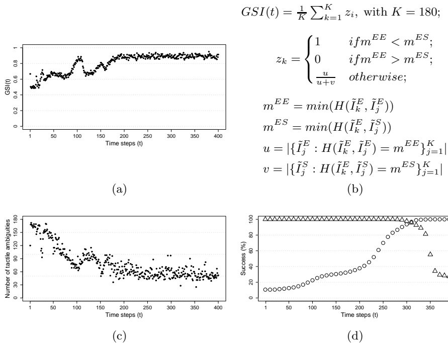
Fig. 2. (a) The Geometric Separability Index (GSI); (b) the formal definition of GSI; (c) the number of tactile ambiguities; (d) the percentage of success in pre-substitution tests (see triangles) and post-substitution tests (see empty circles).
