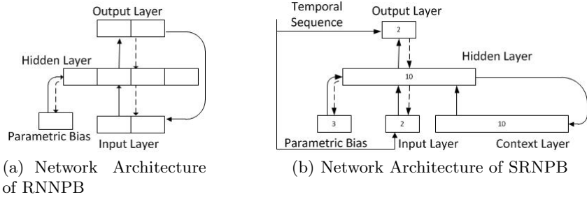
Fig. 1. Comparison of architectures of RNNPB and SRNPN
