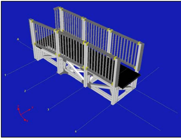
3D model of the Leri Footbridge
