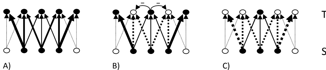
FIGURE 5: Approaches to competitive learning. A) No competitive learning. All neurons in the target s-layer T that can see an active source in the input s-layer S are connected to their inputs. The weight values are represented by the thickness of the connection line, reflecting rule (5). B) Lateral inhibition prevents neighboring neurons in s-layer T from developing their own connections. It is assumed here that the central neuron has been first to fire. C) Effect of pruning the connections in A). Each neuron in s-layer S keeps only the one output connection with the lowest weight. This automatically preserves in s-layer T the neuron with the most representation power, i.e. represents the largest number of active neurons in s-layer S.
