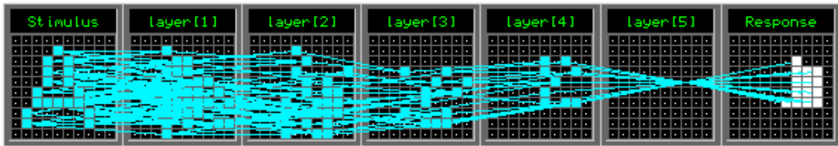
Figure 10: Connection tree developed after 15 training runs with the same A->right hand response SR pair. The network has recruited 4 nodes in layer 5, of which 3 show similarly dense trees. This figure can be compared with the top row of figure 8, showing a large number of redundant connections have been developed. The only difference in network parameters is the synaptic transmission probability p = 0.5 . Simulations of 15 training runs with p=1 produce a single tree, as in the top figure 8.
