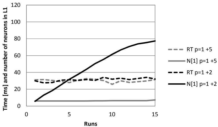
FIGURE 9. Results of repeated learning of the same SR pair, e.g A->Right-hand, for two values of the synaptic transmission probability and of the weight updating delay. A) Synapses are probabilistic, with transmission probability p=0.5 . Weights are either updated at the peak of the alpha function (+2) or in the tail of the alpha function, 3ms after its peak. B) Synapses are deterministic ( p=1 ) with two updating times as in A). The continuous curves marked with N represent the total number of neurons recruited in s-layer 1. The dotted lines represent the response time of the network to presentation of the stimulus after the indicated number of runs.
