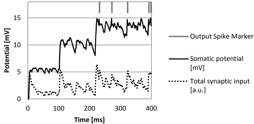
FIGURE 1. Example of the operation of the LIF neuron model used. The synaptic weights are set to W_0/3 , with W_0=7 . Three Poisson inputs (100Hz) start to become active at t=0 , 100 and 200 respectively. Synaptic depression (4) causes the input current to peak when a synapse receives its first spike, then subsequent spikes have a smaller effect. The postsynaptic potential shows the characteristic saturation due to the use of balanced depression, with RC=\tau_{REC}=50ms . The neuron fires when the potential reaches the firing threshold V_{th}=15 mV. It then enters a mode of sustained firing where the neuron produces spikes as a Poisson process with refractory time.
