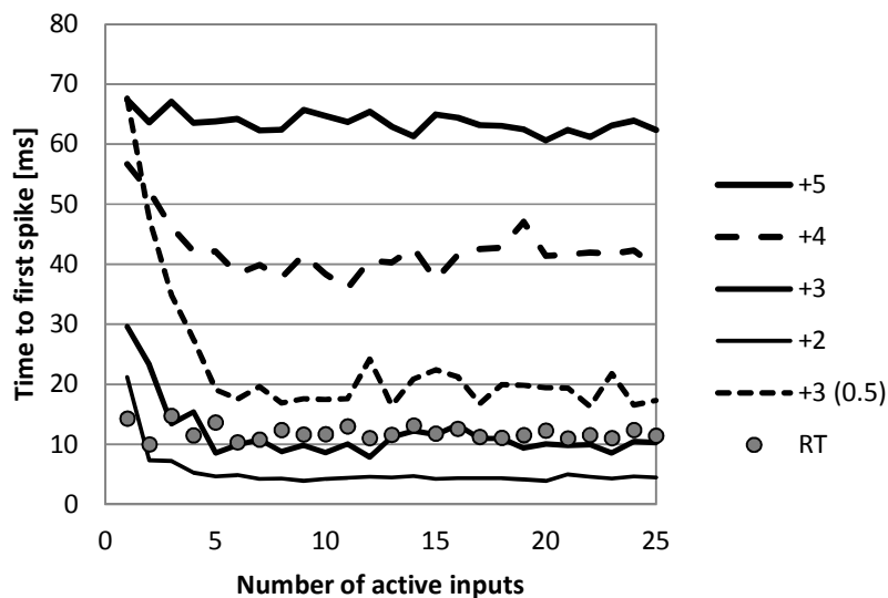
FIGURE 3: Average times to first spike of a leaky integrate-and-fire neuron (LIF) learning to respond to the indicated number of active inputs. Rule (10) was applied with W_0=8 . The curves differ by the delay after spike production when the new weights are becoming effective. The number “+2” means that the weights change at the peak of the alpha function. “+5” means 3ms after the peak. All curves are obtained with \eta =1 , except for one curve with \eta =0.5 (indicated as “+3 0.5”). RT is the response time of a neuron with weights preset to W_0/m . Input spike trains are Poisson spike trains, where the firing probability is set to 100Hz at time 0. The somatic potential and synaptic weights are initially zero.
