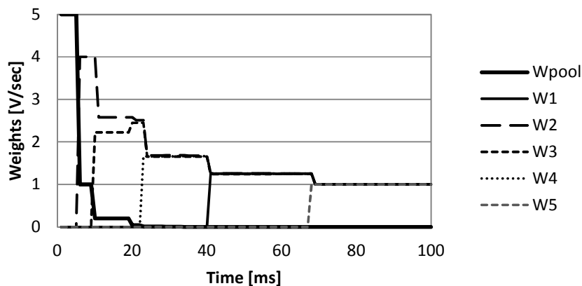
FIGURE 2: Weight learning example with 5 active inputs starting to fire at time 0. All weights are initially zero and are set by the learning procedure described above as soon as the first spike of an input neuron arrives. I used W_0=5 and the final weights are all equal to W_0/5 . The thick line is the quantity of weight W_{POOL} in the store. Each step change in weights corresponds to an input spike arriving on a synapse with a weight that has not reached its final value W_0/m where m is the current number of activated synapses. Inputs are Poisson spike trains firing at 50Hz in this example. \eta = 0.8 .
