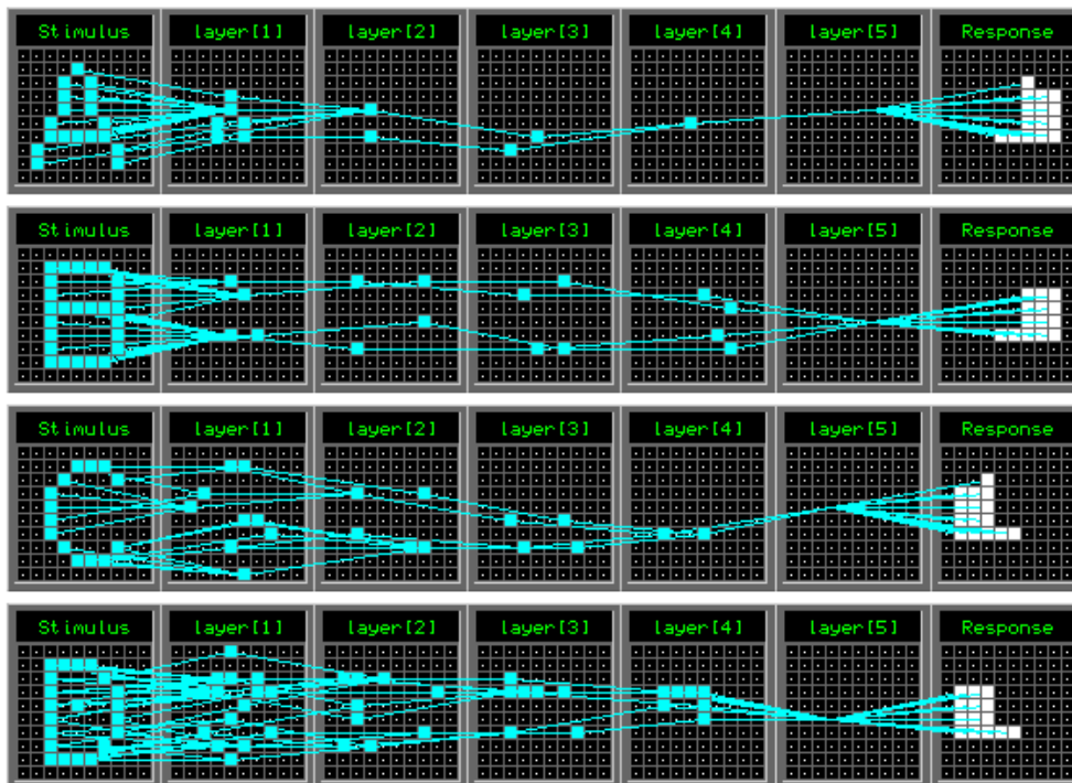
FIGURE 8. Main connection trees developed during training of four stimulus-response associations. A->right hand response, B->right hand response, C-> left hand response, D-> left hand response. Two other trees that link B and D to the “finger tip” of the left and right-hand responses are not shown. Parameters: Synaptic transmission probability=1.0, eta=0.8, weights updates 2 ms after spike arrival, i.e. at the peak of the alpha function. W_0=8 .
