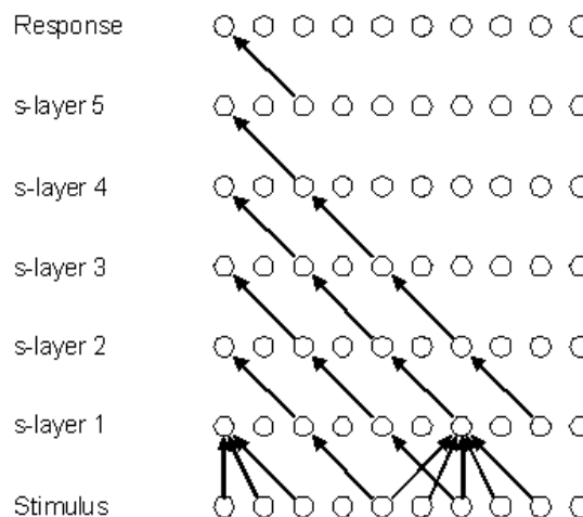
FIGURE 6: Network architecture. Each s-layer is a 10x10 square grid of neurons. Each neuron in an s-layer above Stimulus receives inputs from 5 x 5 neurons. The network is seen from the side.
