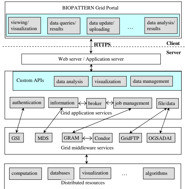
Figure 1. BIOPATTERN Grid Architecture
